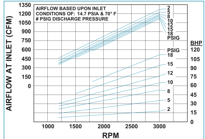
T1055 Pressure Curve
